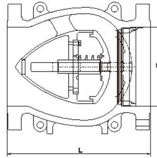
Short pattern
