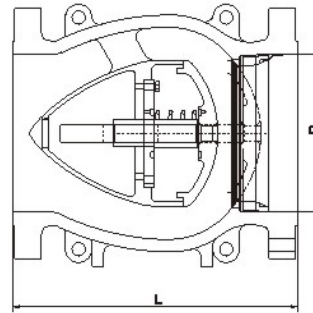
Short pattern
