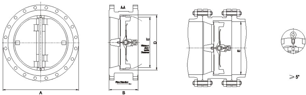
Double flanged type
