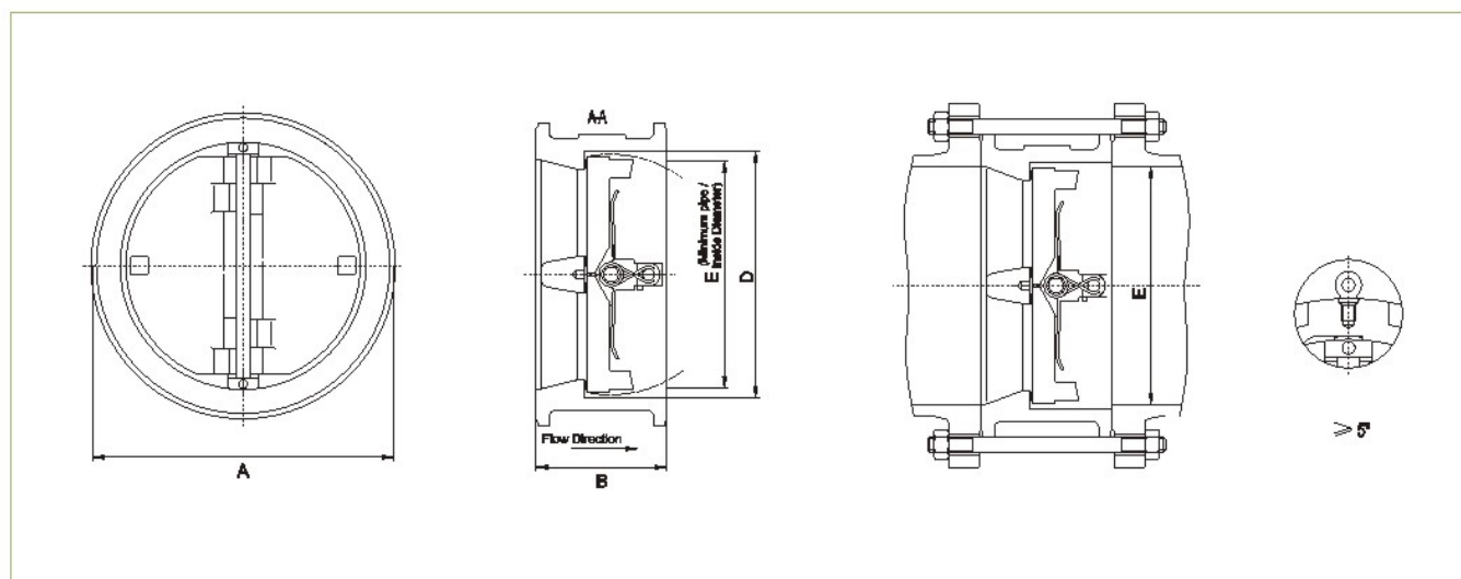
Wafer type
