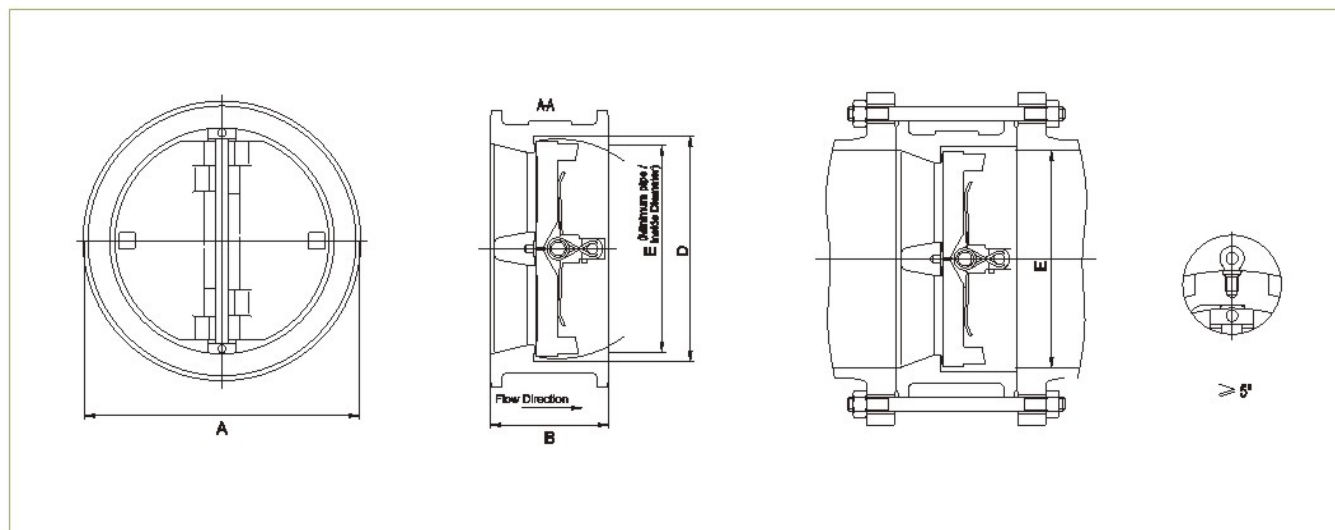
Wafer type
