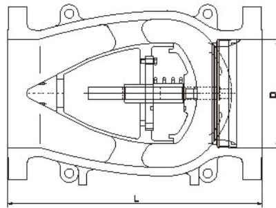
Long pattern
