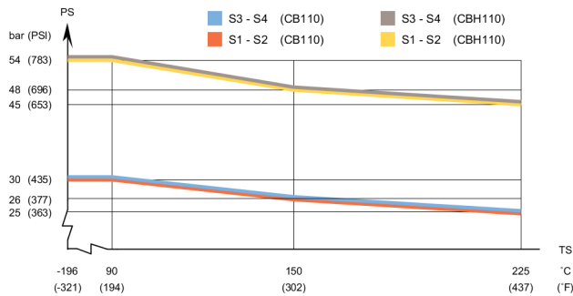
PV code PED pressure/temperature graph
